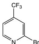
2-Bromo-4-(trifluoromethyl)pyridine
