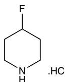
4-Fluoropiperidine hydrochloride
