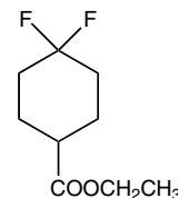
Ethyl-4,4-difluorocyclohexane carboxylate
