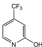
2-Hydroxy-4-(trifluoromethyl)pyridine
